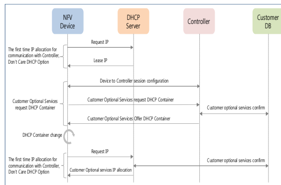
Fig. 7. NFV device's additional service customer DHCP container acquisition process.
