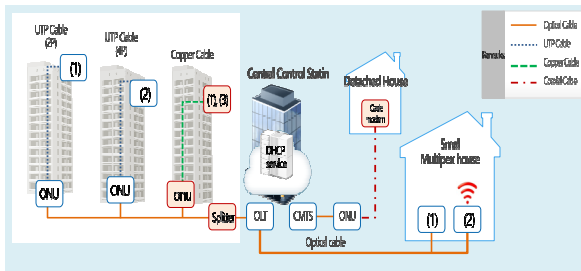
Fig. 1. Wired/wireless communications service network diagram.
