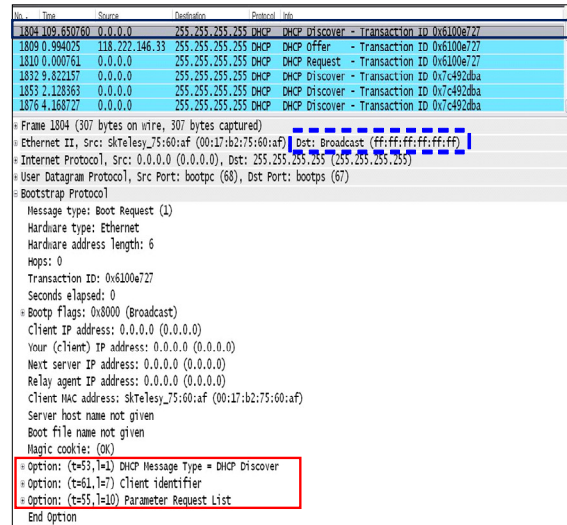
Fig. 2. Option field in DHCP Discover.
