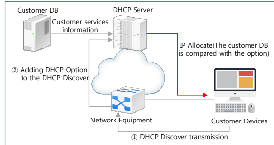
Fig. 3. DHCP option operation in subscriber equipment ONU structure.
